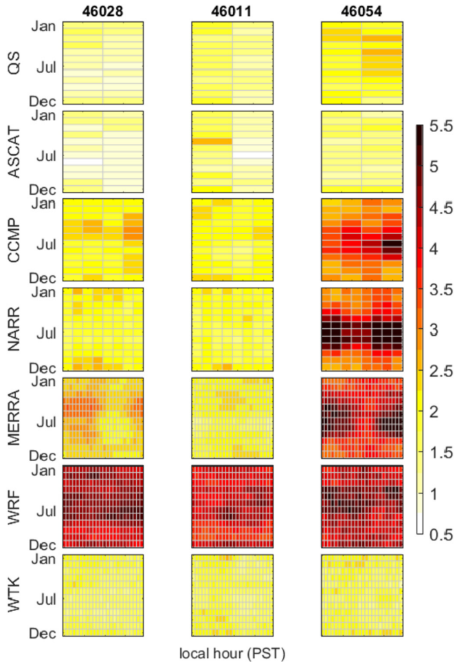
Fig. 6. Similar to Fig. 5, but for root-mean-squared error in the hourly near-surface wind speed in each month ( \text{m s}^{-1} ).
