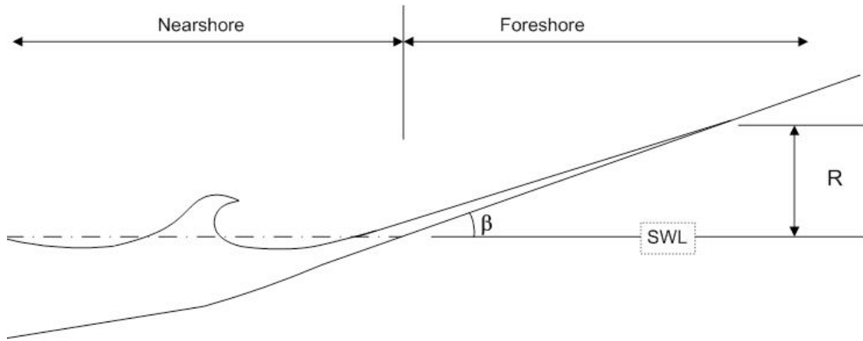
Figure 3.5. Schematic representation of the runup of waves on a beach
