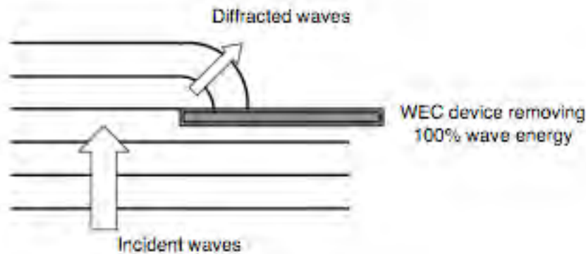
Figure 3.4. Schematic of diffraction of waves into the wave shadow behind a WEC device (or breakwater) that extracts 100% of the incident wave energy.
