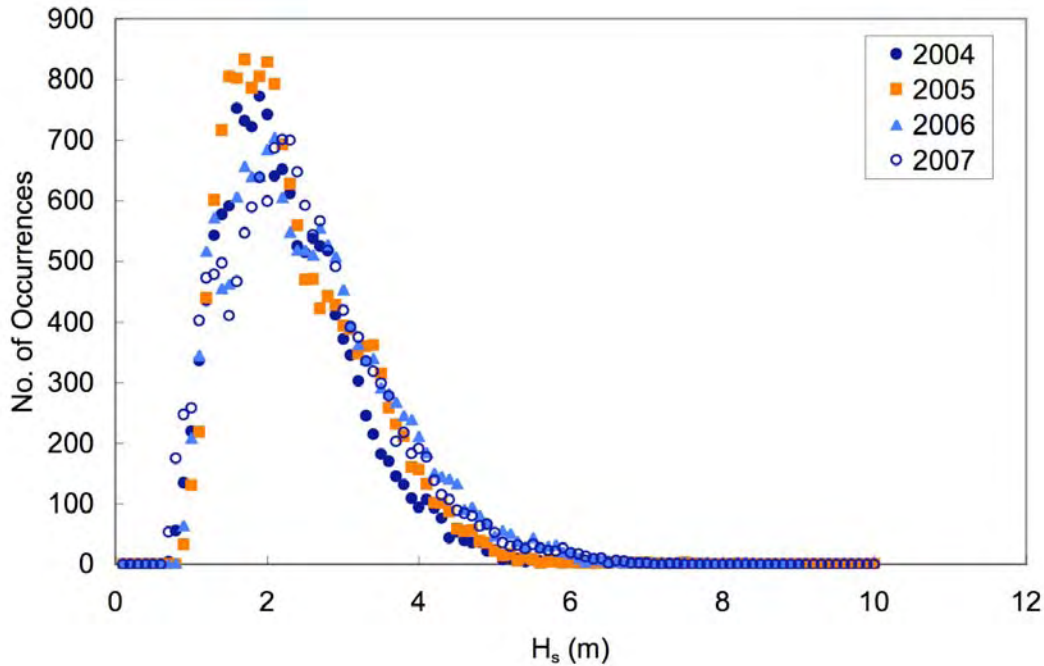
Figure 3.3. The distribution of significant wave height H_s for the years 2004 to 2007 at the CDIP Pt Reyes Buoy.
