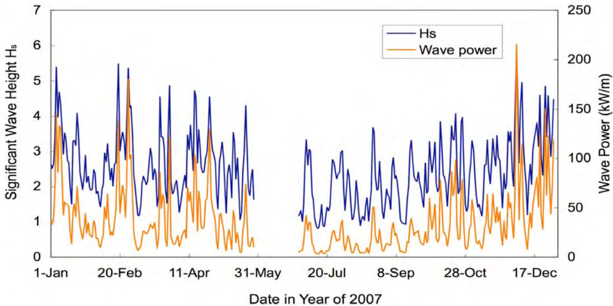
Figure 3.2. Daily average significant wave height H_s (m, blue line) and wave power (kW/m, orange line) observed at CDIP Pt Reyes Buoy in 2007
