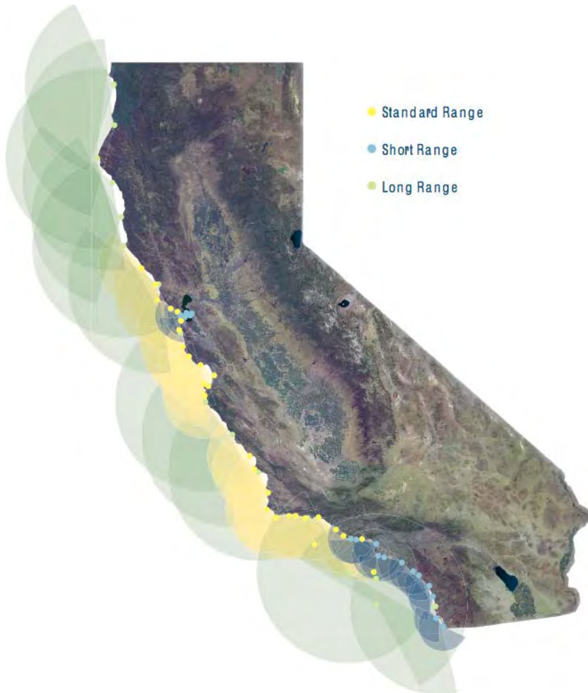
Figure 7.4. Map of the planned high-frequency radar coverage for California, as a part of the state's COCMP (Coastal Ocean Current Monitoring Program)
