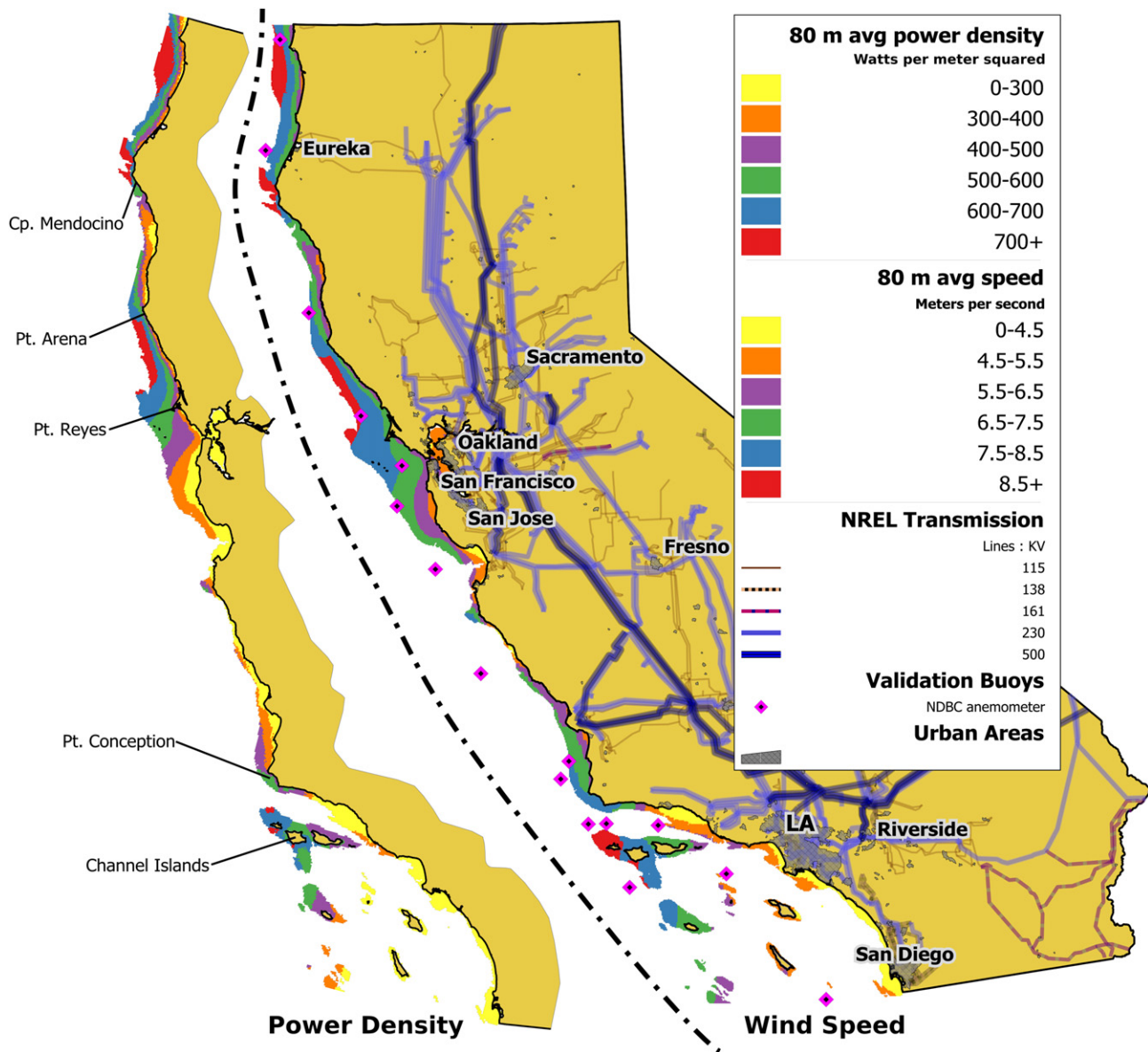
Fig. 2. Modeled 80 m average power density (left) and wind speed (right), based on seasonal 2005/2006 and complete 2007 MM5 winds. The wind resource corresponding to 0–200 m depth is shown. Locations where \bar{v}_{80\text{ m}} \geq 7.5\text{ ms}^{-1} and 7.0\text{ ms}^{-1} were considered in this study. Urban areas highlight where the electricity demand exists. Transmission lines show where offshore wind farms could connect to the existing grid infrastructure.
