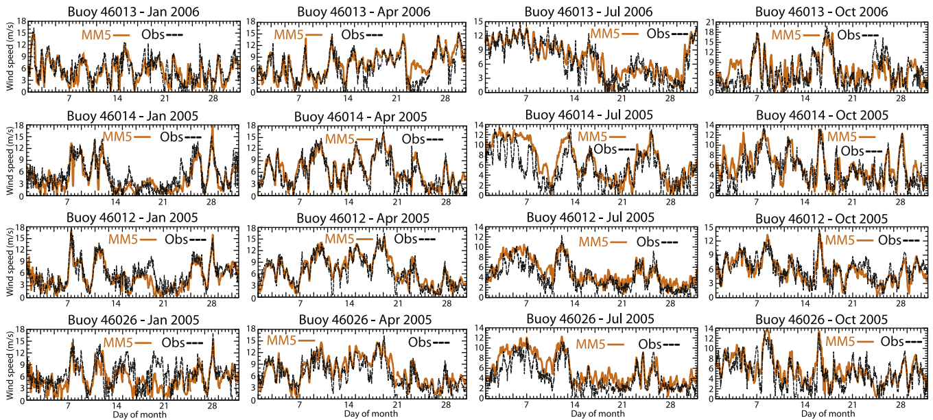
Fig. 3. 16-Months of representative 10 m height MM5 winds and the 5 m height NDBC buoy winds. The first two rows are from Domain 1 (5 km resolution, CA inclusive) and the last two rows are from Domain 2 (1.67 km resolution, San Francisco Bay Area). Buoy station number and year-month are indicated on each individual. See Fig. 2 for location of the NDBC buoys.
