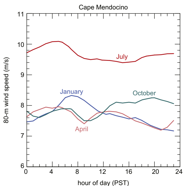
Fig. 5. Mean \bar{v}_{80\text{ m}} winds group by hour of the day (PST) for the proposed wind farm off the NCA coast (Fig. 4), based on the MM5 output for the 2005/2006 months of January, April, July, and October.
